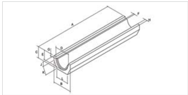
FIG. 3 Typical Rebated channel
