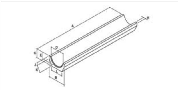
FIG. 1 Typical Half round channel (no rebate)
