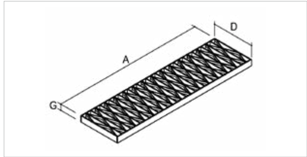
FIG. 2 Grate
