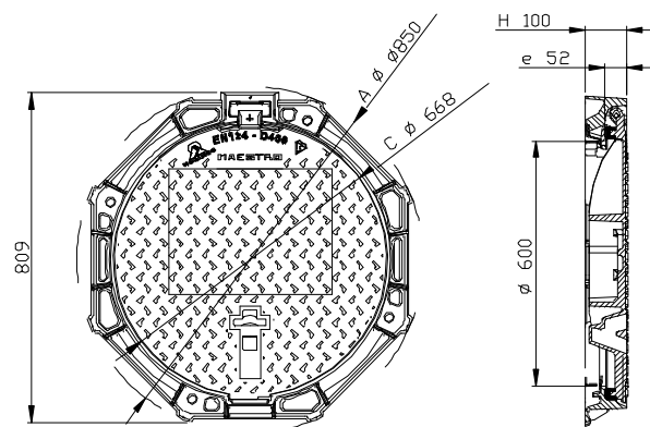
FIG. 1 Product Dimensions
