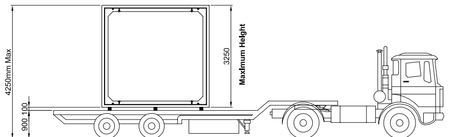
LOW BED TRAILER - SIDE ELEVATION
