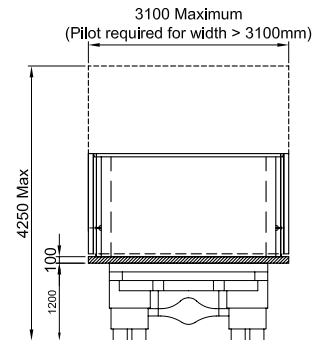
STANDARD TRAILER - END ELEVATION (BACK)
