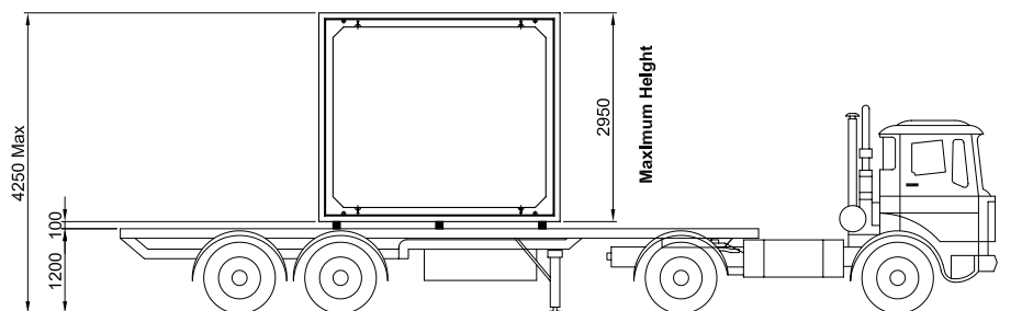
STANDARD TRAILER - SIDE ELEVATION
